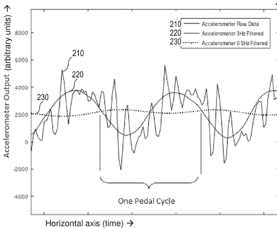
VERTICAL-AXIS ACCELEROMETER DETECTING ONE PEDAL CYCLE
