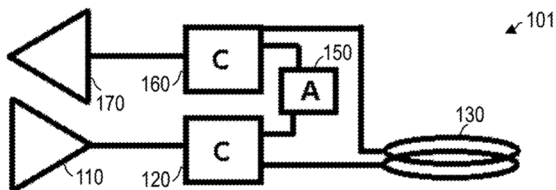
FIG. 1C (Block diagram)
