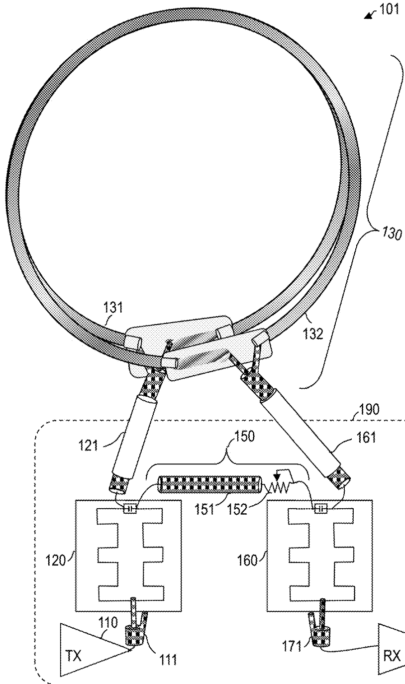
FIG. 1A (Front view)
